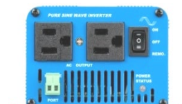
Inverter 12/180 with Nema 5-15R sockets
